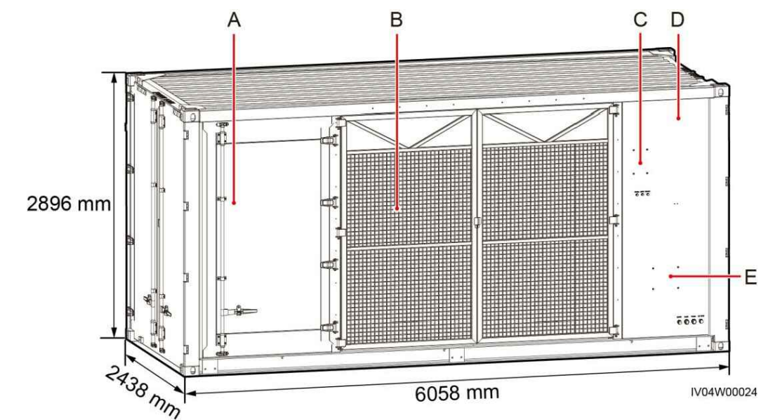
(A) LOW-VOLTAGE ROOM (LV) (B) TRANSFORMER ROOM (TR) (C) INSTALLATION POSITION FOR THE DISTRIBUTED POWER SYSTEM (D) MEDIUM-VOLTAGE ROOM (MV) (E) INSTALLATION POSITION FOR THE SMART ARRAY CONTROLLER
