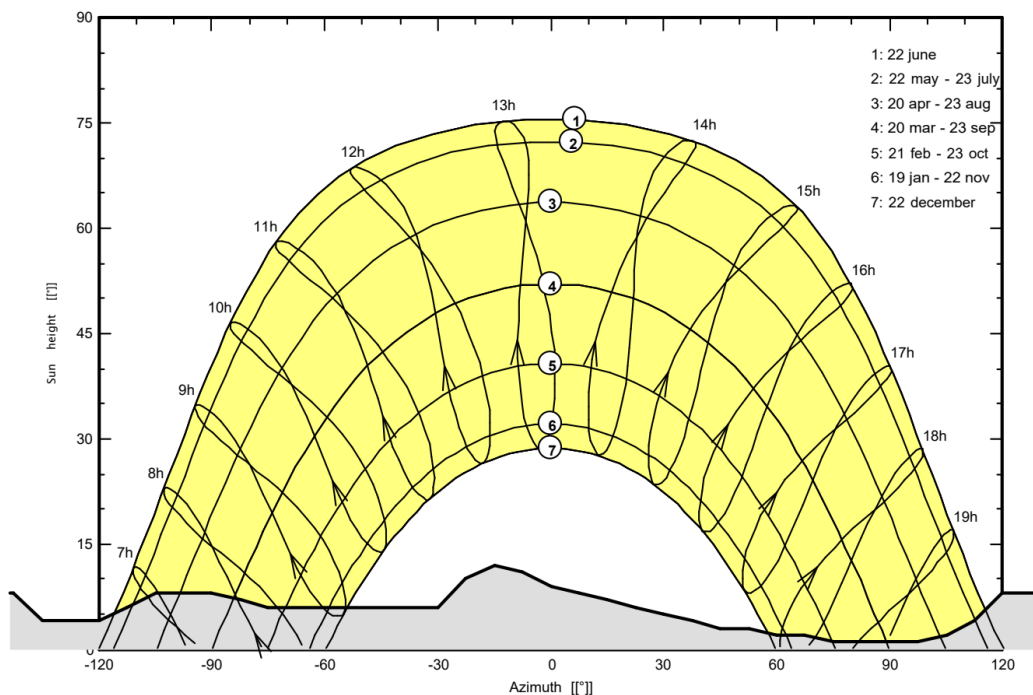
Horizon from PVGIS website API, Lat=37°51'32', Long=-3°5'26', Alt=564m
