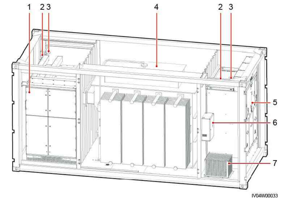
(1) LOW-VOLTAGE CABINET (2) LIGHT (3) SMOKE SENSOR (4) TRANSFORMER (5) RING MAIN UNIT (6) POWER DISTRIBUTION BOX (7) AUXILIARY TRANSFORMER
