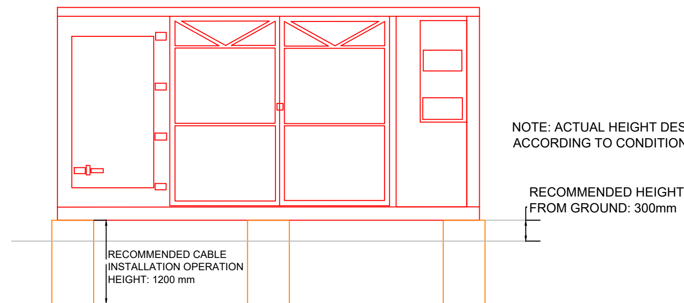
FOUNDATION DIMENSIONS
