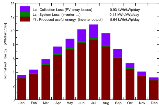
Normalized productions (per installed kWp): Nominal power 1187 kWp
