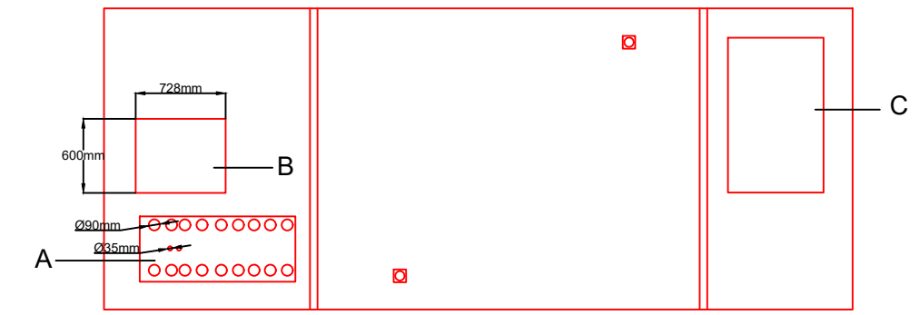
(A) AC INPUT POWER CABLE HOLE (B) TRENCH ENTRY (C) PRESSURE RELIEF CHANNEL AND CABLE HOLE (RING MAIN UNIT)
