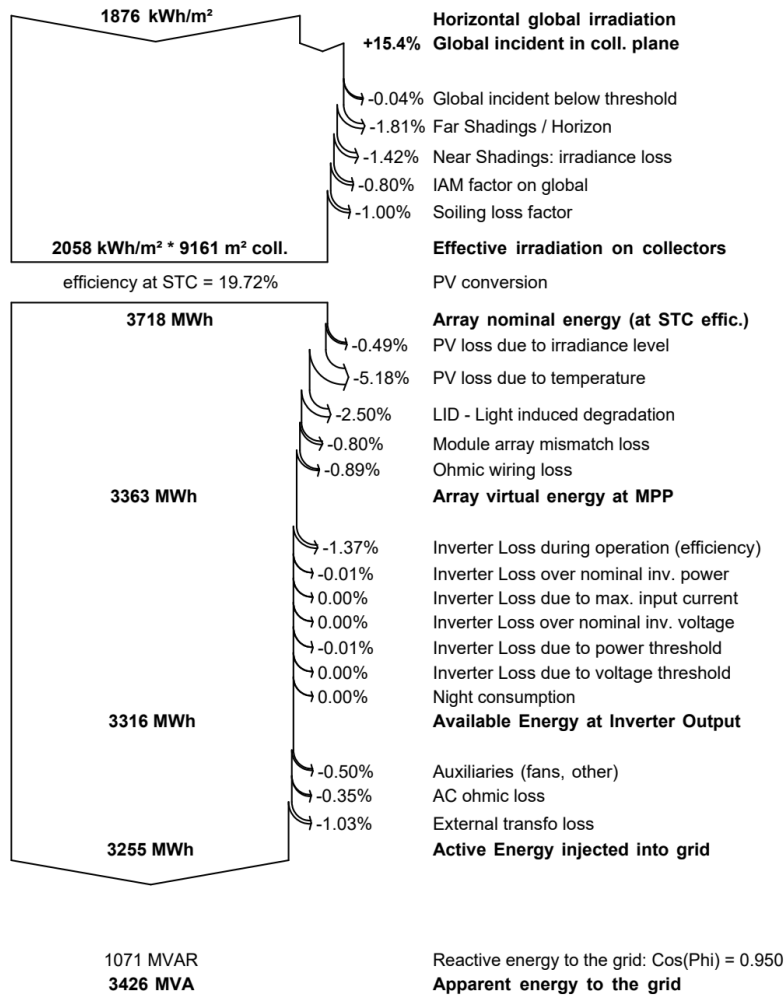
Loss diagram over the whole year
