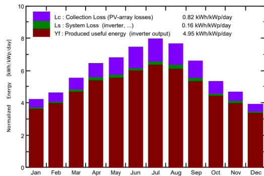
Normalized productions (per installed kWp): Nominal power 1803 kWp
