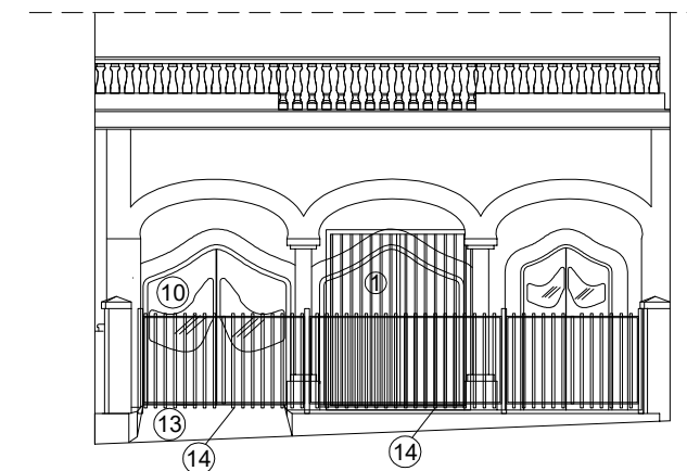
ALZADO PRINCIPAL
