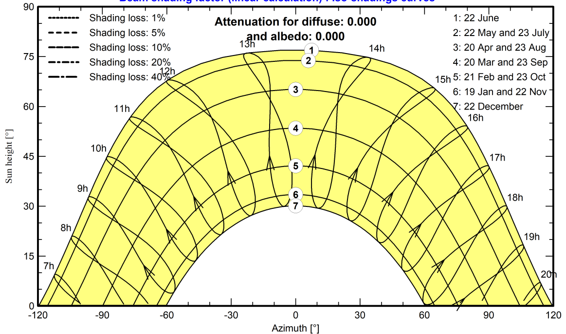
Beam shading factor (linear calculation) : Iso-shadings curves
