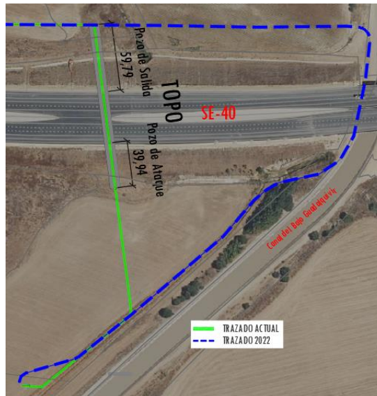
Imagen1: Topo SE-40
