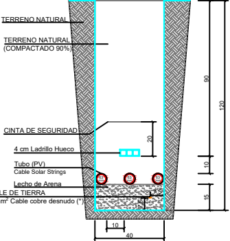
CC(A) 40x111 cm
