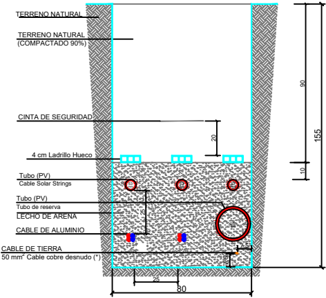
Max. 2 circuitos Al CA(B.1) 80x155 cm
