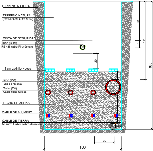
Max. 4 circuitos de Al CC(B.2) BUSES 100x165 cm.
