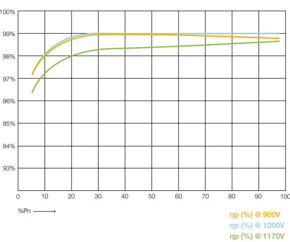
Efficiency PV 2500
