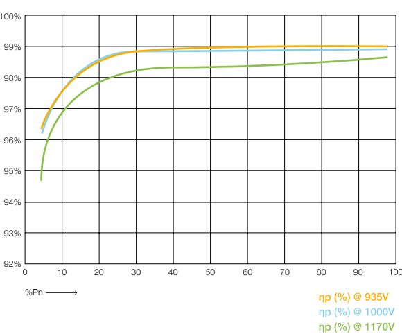
Efficiency PV 2250
