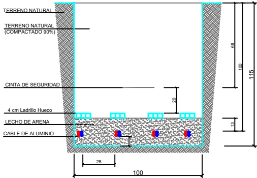
Solo 4 Circuitos de Al CC(B.3) 100x112 cm
