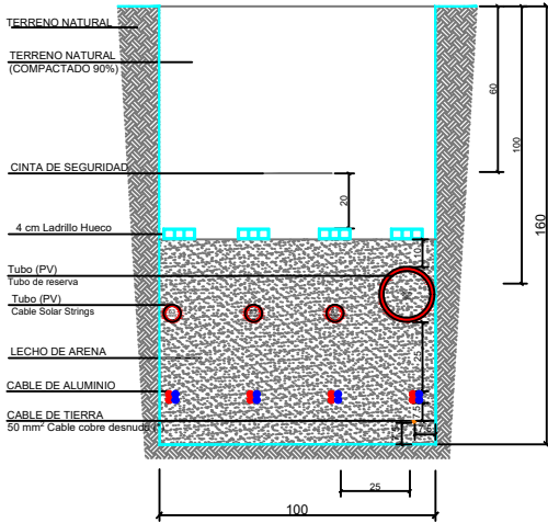
Max. 4 circuitos de Al CA(B.2) 100x160 cm
