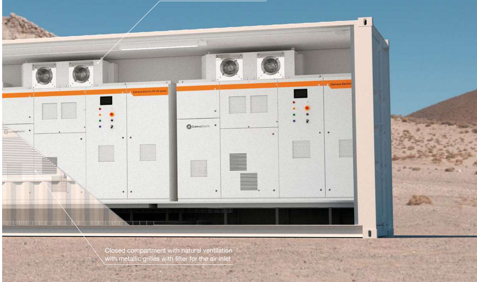
Gamesa Electric PV 2X series inverters with liquid/air active cooling
